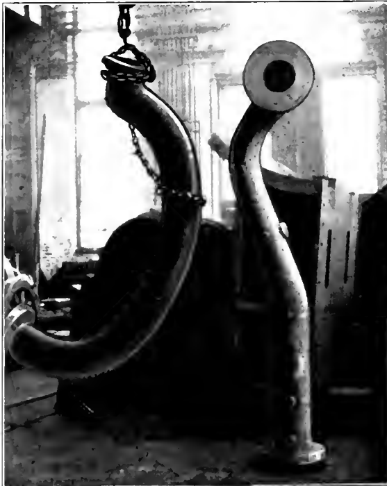
Fig. 1.—Castings from Which the Steam Pipes for the Superheater Locomotive Were Made
